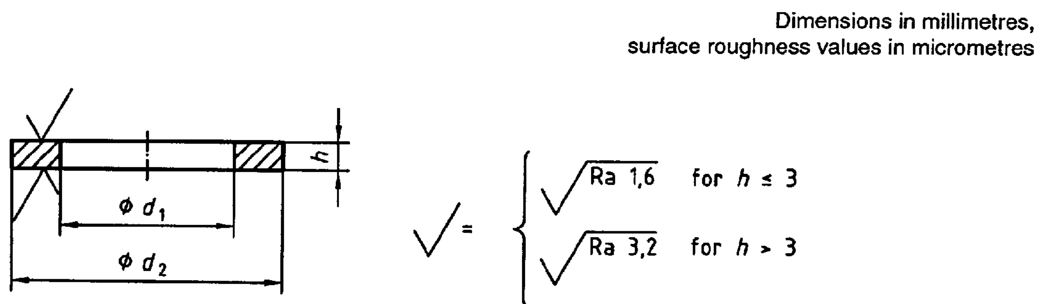
Figure 1 — Dimensions
